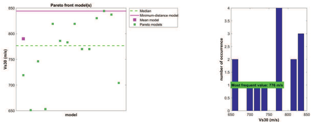
Figura 58: Correlazione Vs30 median, minimum-distance model, mean model, pareto models
