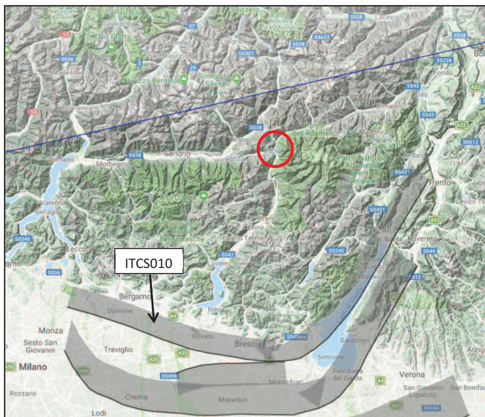
Figura 3: Stralcio The European Database of Seismogenic Faults" (SHARE task 3.2)
