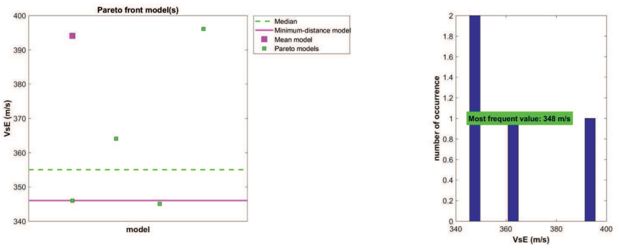
Figura 44: Correlazione VsE median, minimum-distance model, mean model, pareto models
