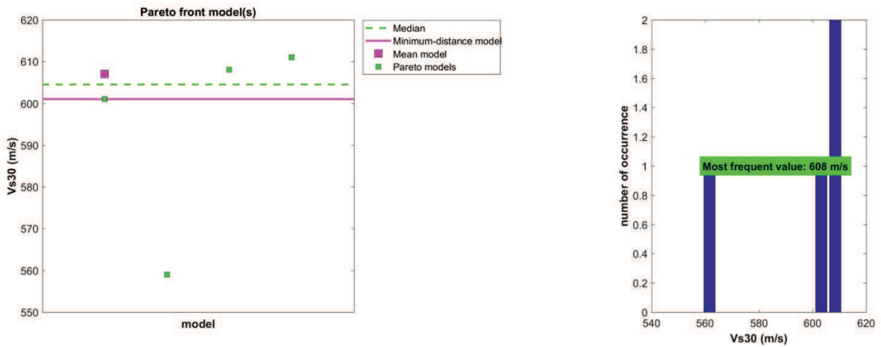
Figura 43: Correlazione Vs30 median, minimum-distance model, mean model, pareto models
