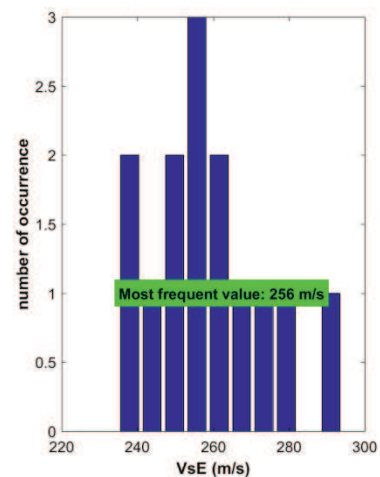
Figura 59: Correlazione VsE median, minimum-distance model, mean model, pareto models
