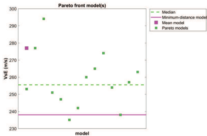
Figura 59: Correlazione VsE median, minimum-distance model, mean model, pareto models
